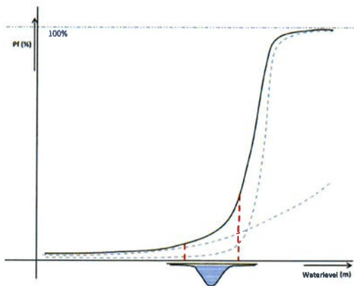
Figure 16: Calculating flooding-probabilities: integrating forecast-distributions under the fragility-curve.
