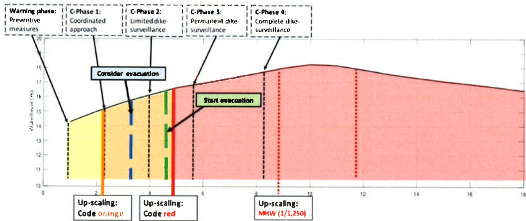
Figure 18: Comparison of current emergency-procedures with the calculated alarm-waterlevel to call for evacuation (MHW is defined as the water level with a return period of 1250 years).
